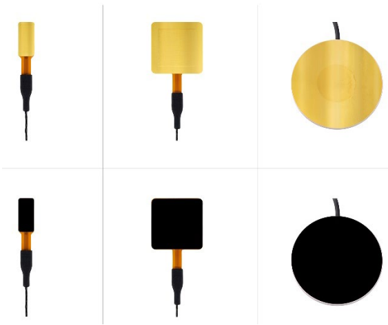
Figure 1 BLK – GLD stickers with radiation-absorbing (black) and -reflecting (gold) coatings are available for FHF05(SC) series and HFP01 heat flux sensors
