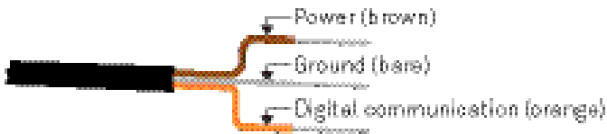
Figure 2 Pigtail wiring
