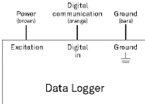
Figure 3 Wiring diagram
