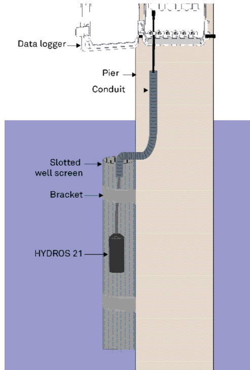
Sensor suspended in water body
